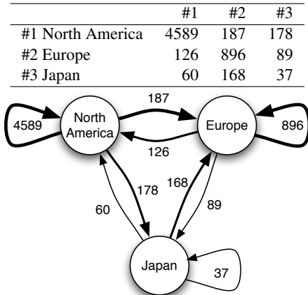
Figure 3. World trade: \mathbf{R} matrix from NN-ASALSAN and associated graph showing aggregate trade patterns.
