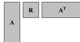
Figure 1. Two-way DEDICOM model.
