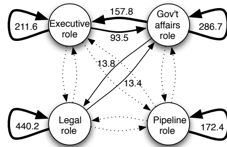
Figure 6. Enron corpus: R matrix and associated graph showing aggregate communication patterns.
