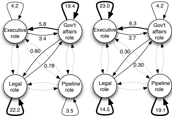
Figure 8. Graphs of D_k R D_k showing communication patterns for k = October 2000 (pre-crisis, left) and k = October 2001 (during crisis, right).
