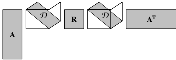
Figure 2. Three-way DEDICOM model.
